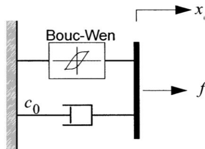
Figure 1. Mechanical model of MR damper [36]
