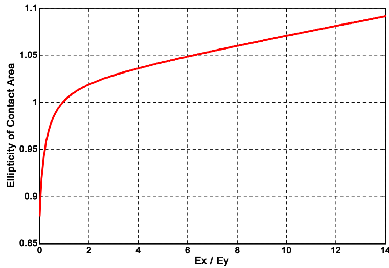
Fig. 4. The elliptic treatment of contact area between bodies
