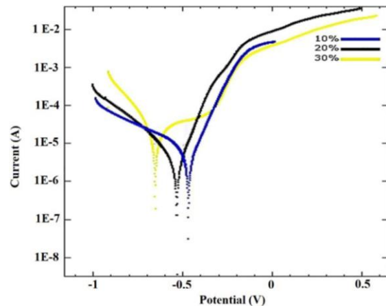
Fig. 7. Tafel curves of the coatings prepared at a current density of 0.2 A/cm 2 , a frequency of 10 Hz and with different duty cycles in a 3.5% NaCl aqueous solution
