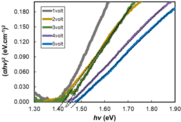
Fig. 8. Band Gap sample using Tauc-Plot
