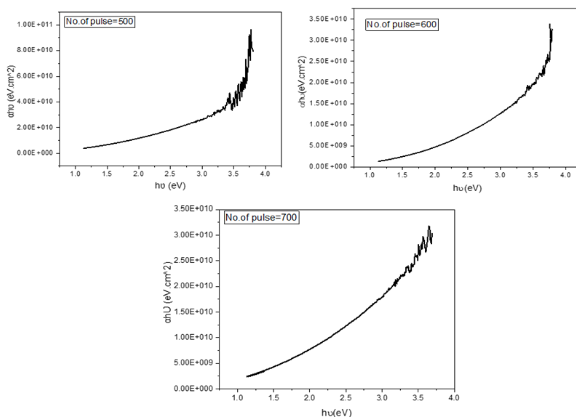
Fig. 7. Optical energy gap of the TiO 2 /MgO nanocomposite at various numbers of laser shots.
