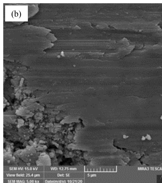
Fig. 21. Image of the sample surface (a) The sample with the lowest hardness (351170) and (b) The sample with the highest hardness (350550) after performing an abrasion test at a constant load of 300 g force and a distance of 50 meters.
