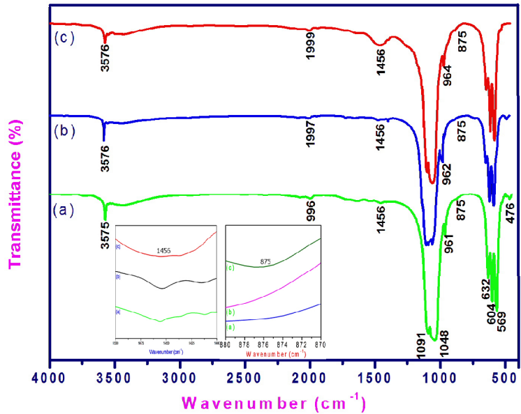
Fig. 2. FTIR spectra of the HAp-C (a), HAp/PEG-C (b) and HAp/PVP-C (c) at 900 °C. Inset shows magnified image of peaks at 875 and 1456 \text{cm}^{-1} .
