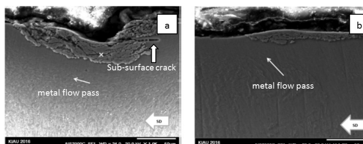
Fig. 8. SEM micrographs of under-worn surface of the samples in this study. a) 930°C air quenched and b) 930°C water quenched
