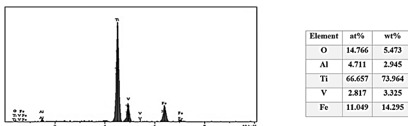
Fig. 9. EDS microanalysis results of MML layer formed on the worn surface.
