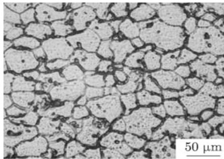
(a) As-weld (before optimizing)
