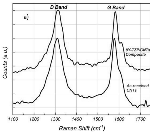
Fig. 4. Raman Spectra of as-received CNTs and as-sintered Z-7.6C composite (a) and X-ray diffraction pattern of 8YSZ nanopowders compared to the sintered Z-7.6C sample (samples have been sintered at 1350°C).
