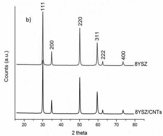
Fig. 4. Raman Spectra of as-received CNTs and as-sintered Z-7.6C composite (a) and X-ray diffraction pattern of 8YSZ nanopowders compared to the sintered Z-7.6C sample (samples have been sintered at 1350°C).
