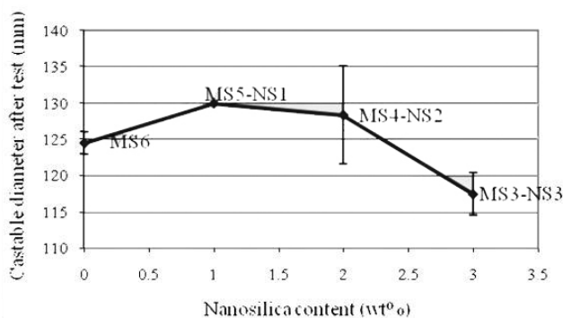
Fig. 1. Castable flowability as a function of nanosilica content
