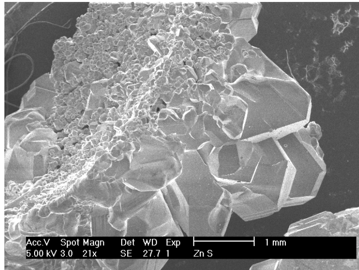
Fig. 9. Spurious nucleation of ZnS crystals at 1102 °C.
