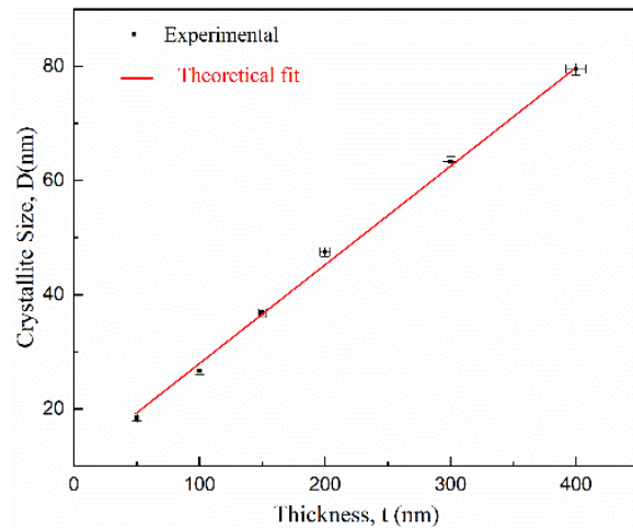
Fig. 3. Crystallite size as a function of Co thickness
