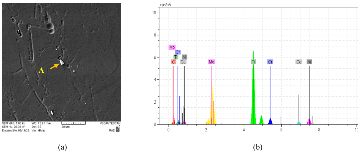
Fig. 3. Secondary phase in base metal a) micrograph b) EDS spectrum result of phase A
