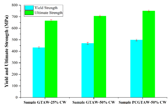
Fig. 9. Comparison of yield and tensile strength of GTAW samples with 25% and 50% pre-cold work levels and the PCGTAW sample with pulsed current welding parameters
