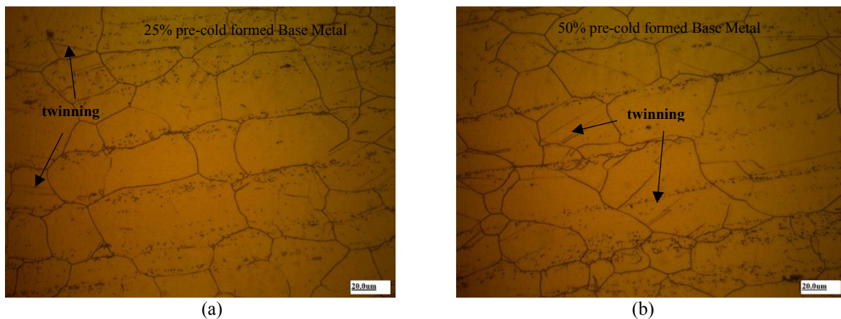
Fig. 2. Optical microstructure of the base metal of Nimonic 80A in a) after 25% CW, b) after 50% CW
