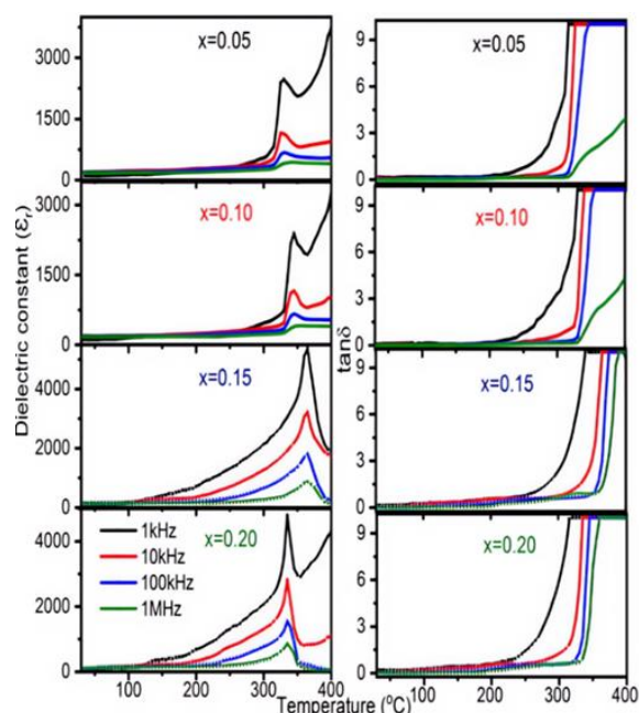
Fig. 7. Temperature dependence of \epsilon' and \tan\delta for (1-y)\text{Bi}_{1-x}\text{Nd}_x\text{FeO}_3-y\text{PbTiO}_3 solid solutions with y = 0.3 and different x compositions in 1 kHz-1 MHz frequency range
