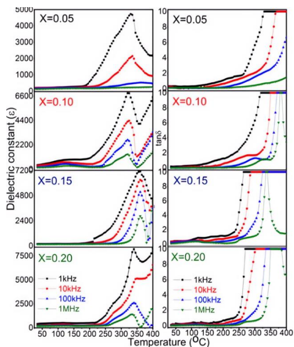
Fig. 5. Temperature dependence of \epsilon' and \tan\delta for (1-y)\text{Bi}_{1-x}\text{Nd}_x\text{FeO}_3-y\text{PbTiO}_3 solid solutions with y = 0.1 and different x compositions in 1 kHz-1 MHz frequency range
