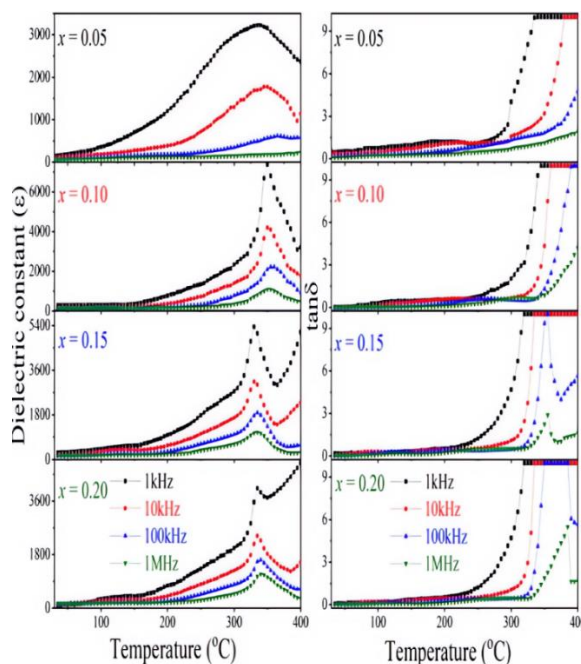
Fig. 8. Temperature dependence of \epsilon' and \tan\delta for (1-y)\text{Bi}_{1-x}\text{Nd}_x\text{FeO}_3-y\text{PbTiO}_3 solid solutions with y = 0.4 and different x compositions in 1 kHz-1 MHz frequency range
