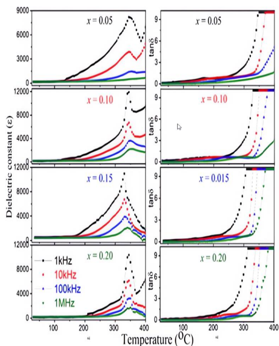
Fig. 6. Temperature dependence of \epsilon' and \tan\delta for (1-y)\text{Bi}_{1-x}\text{Nd}_x\text{FeO}_3-y\text{PbTiO}_3 solid solutions with y = 0.2 and different x compositions in 1 kHz-1 MHz frequency range
