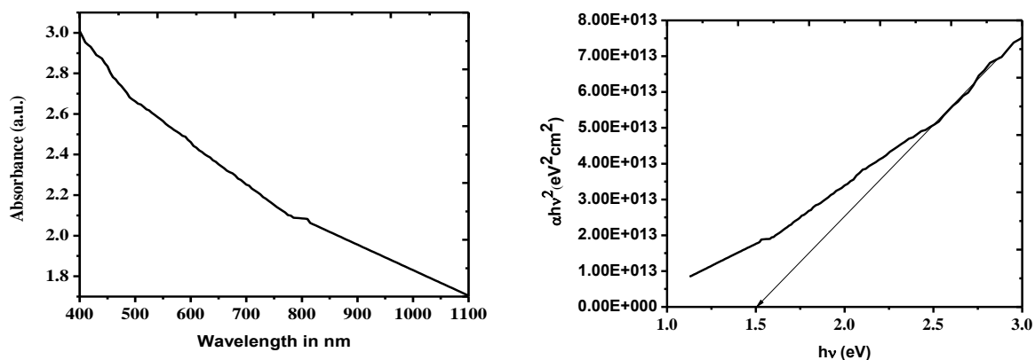
Fig. 6. a) Optical absorption spectrum of CZTS thin film; b) Plot of (\alpha hv)^2 vs h\nu of CZTS thin films.
