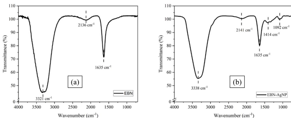
Fig. 3. ATR-FTIR spectra data of (a) EBN extract and (b) synthesized of EBN-AgNPs.
