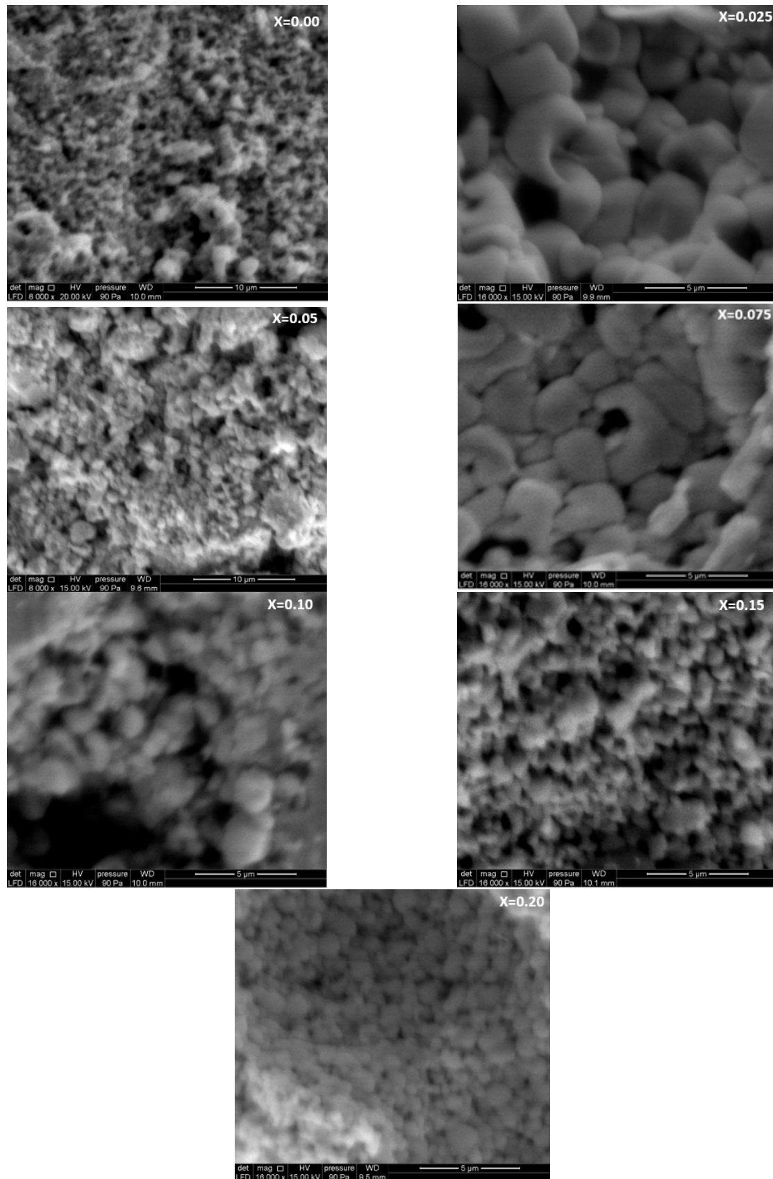
Fig. 4. SEM micrographs of PFZT ceramics for 0.00 \leq x \leq 0.20 sintered at 1100^{\circ}\text{C} for 4 h.
