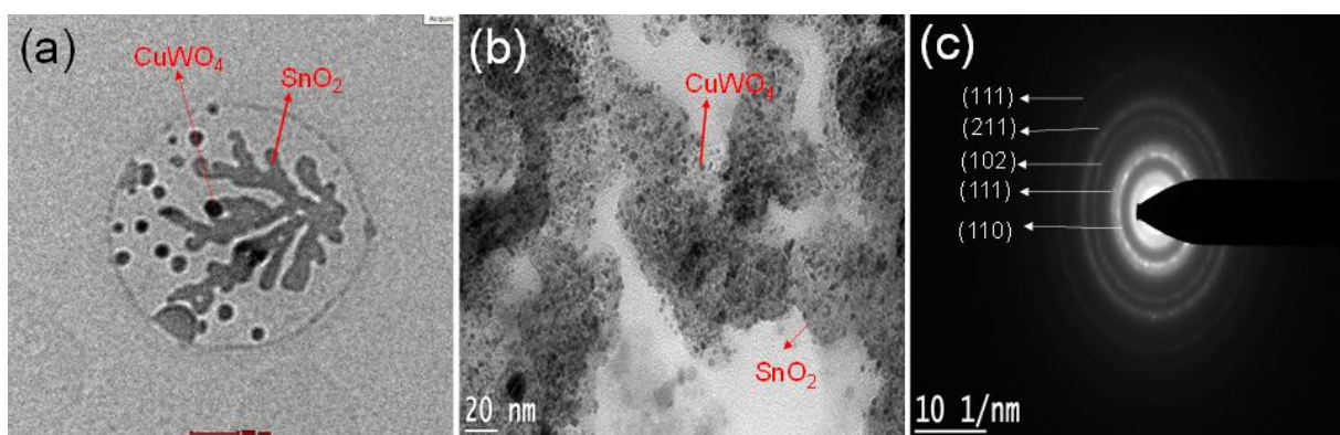
Fig. 4. (a) TEM micrographs (b) HR-TEM (c) SAED pattern of CuWO 4 /SnO 2 .
