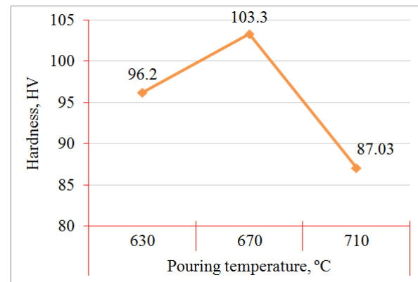
Fig. 11. Hardness plot of three composites
