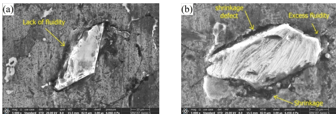
Fig. 8. SEM images of composites prepared at pouring temperatures (a) 630°C and (b) 710°C showing interface formed between particle and Al matrix
