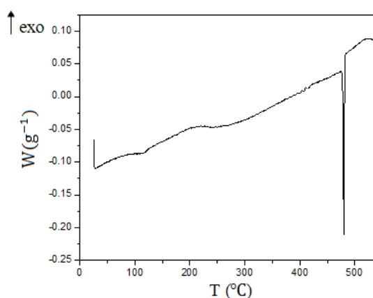
Fig.2. The result of the DSC analysis on a sample of casting 7075 alloy (heating rate: 5°C / min).
