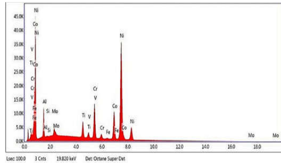
Fig. 24. EDS spectrum of selected area 3
