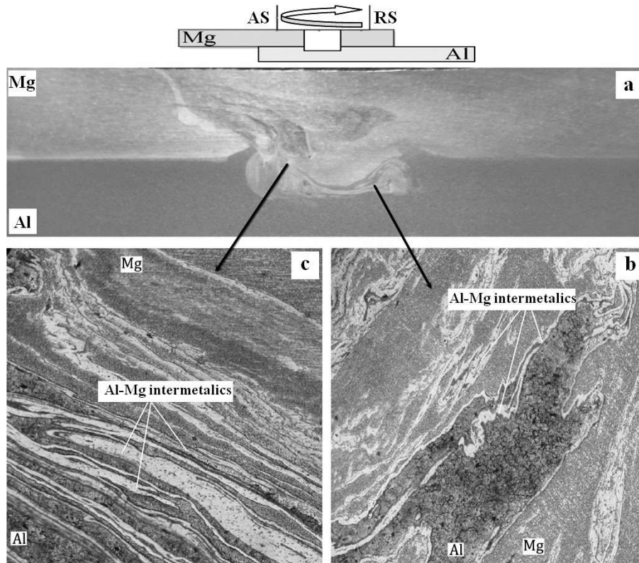
Fig. 9. Microstructure of various regions of dissimilar Al-Mg joint, under the welding condition of 1600 rpm and 40 mm/min (a-c), representing each region of the weld zone marked in macrographs.
