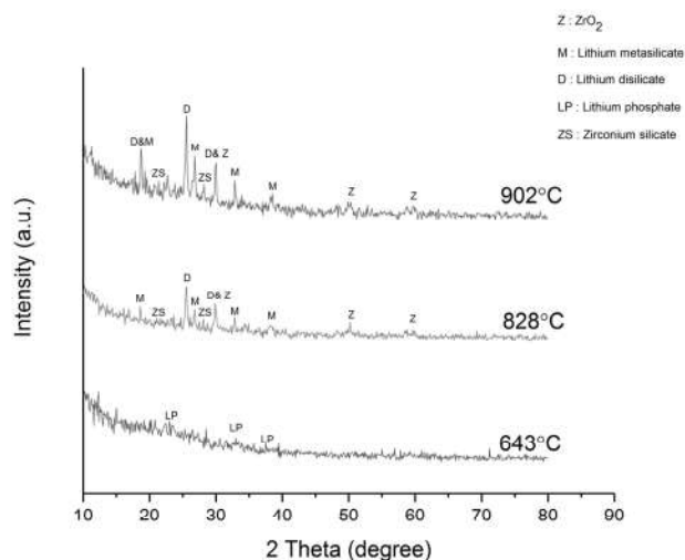
Fig. 3. XRD patterns of glass P 5 after heat-treatment for 1 h at each exothermic peak temperature
