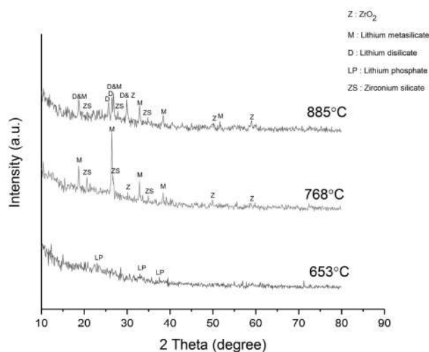
Fig. 2. XRD patterns of glass P 2 after heat-treatment for 1 h at each exothermic peak temperature
