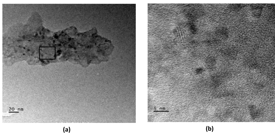
Fig. 7. Transmission electron micrographs of KNN powders calcined at 900 °C for 5h, at lower magnification (a) 20nm and higher magnification (b) 5nm.
