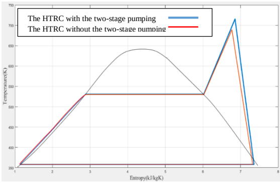
Figure 4. The T-S plot of the HTRC with and without the two-stage pumping.
