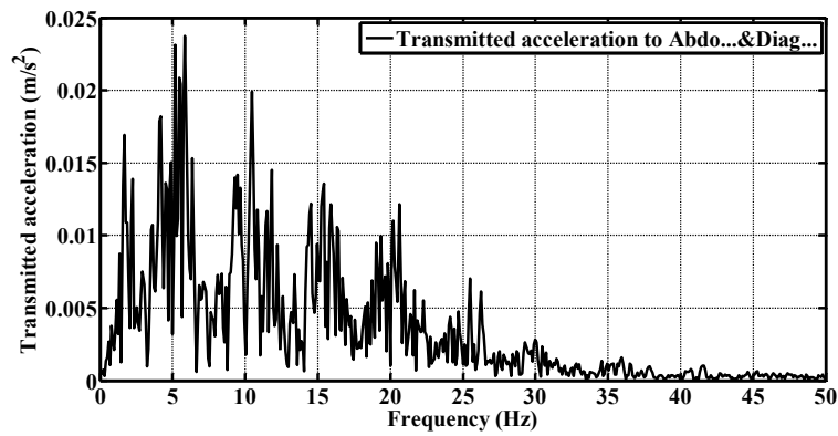
Fig16. Transmitted accelerations to abdomen & diaphragm due to D road profile
