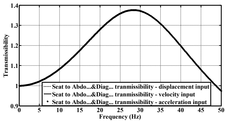
Fig28. Seat to abdomen &amp; diaphragm transmissibility
