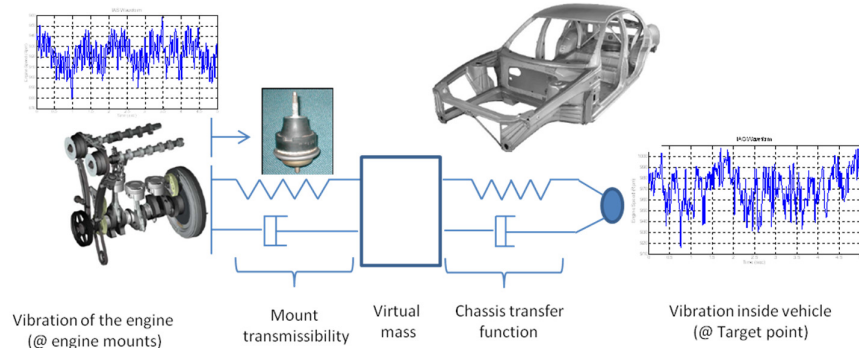
Fig1. Graphical representation of VIVS method
